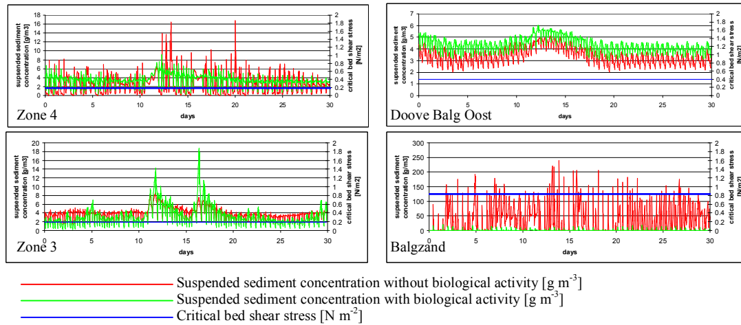
Figure 5-1: Overview of suspended sediment concentration [ \text{g m}^{-3} ] on different places during a summer month (June). The blue lines indicate the critical bed shear stress, >0.4 \text{ N m}^{-2} stabilising, <0.4 \text{ N m}^{-2} destabilising.
