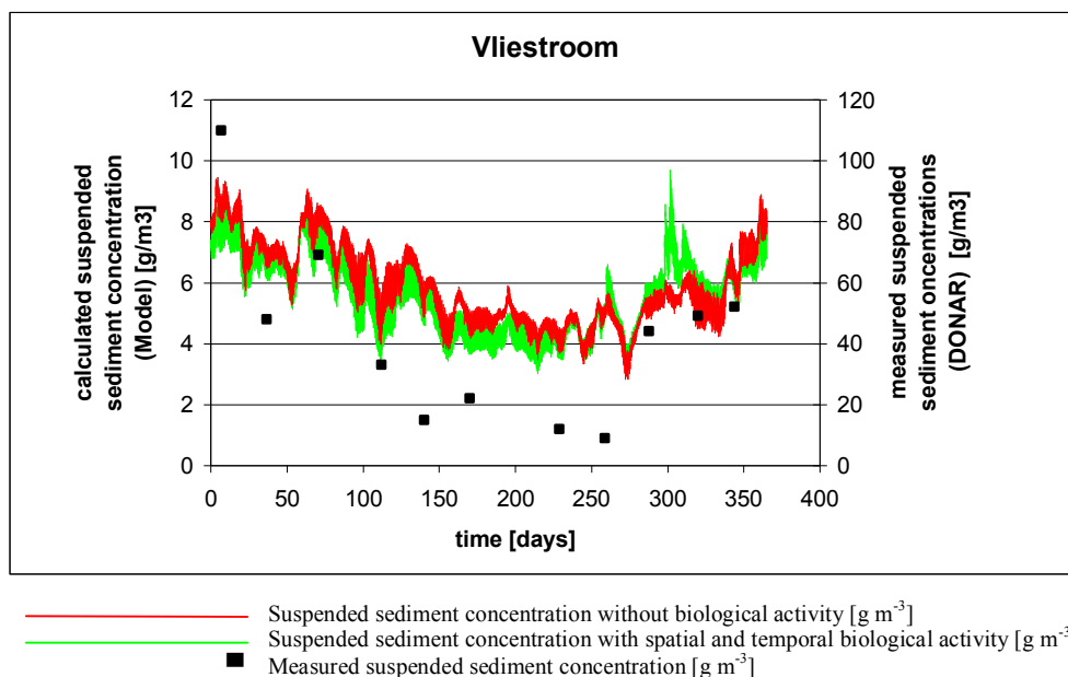
Figure 5-9: Comparison between the calculated suspended sediment concentrations and the measured suspended sediment concentrations [ \text{g m}^{-3} ] (DONAR).
