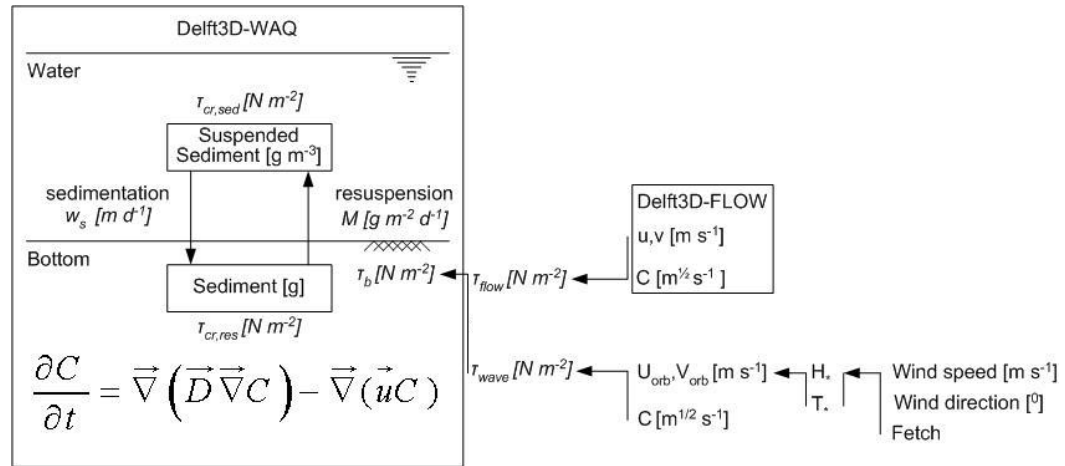
Figure A-1: Connection between the two modules and used parameters.
